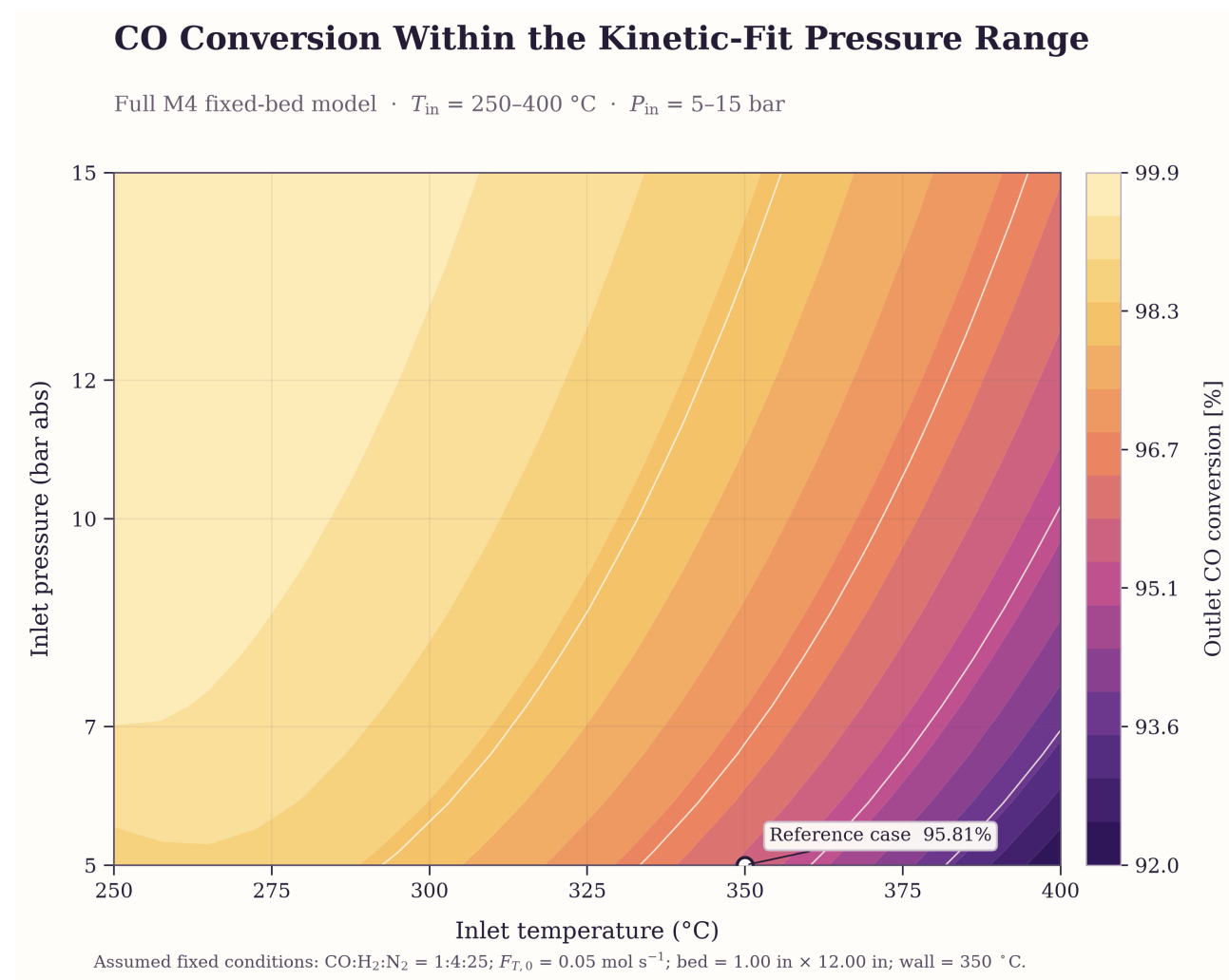
Figure 6. Full M4 sensitivity restricted to inlet pressures of 5–15 bar.
