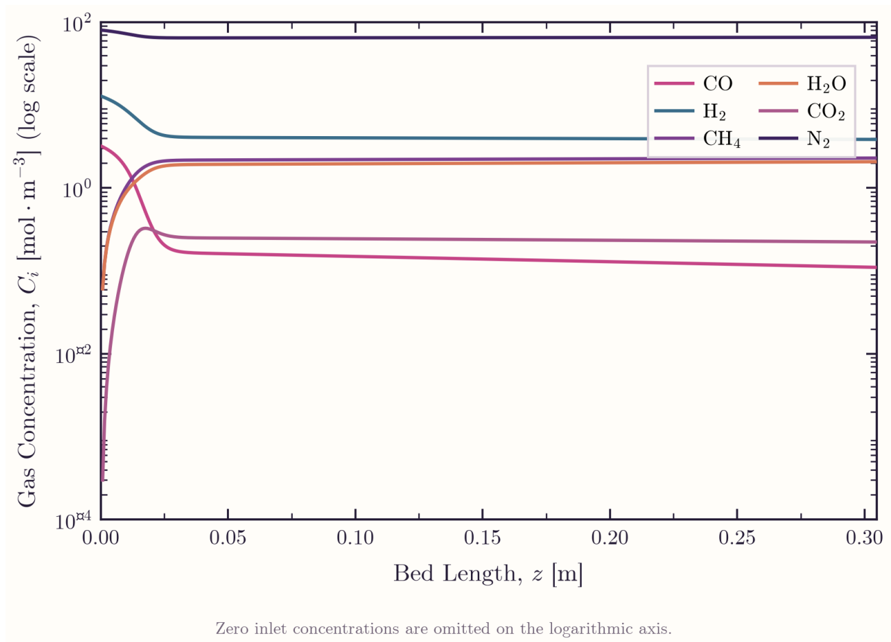
Figure 4. Full M4 species concentrations versus bed length for the assumed 5-bar, 350 °C, CO:H 2 :N 2 = 1:4:25 case.
