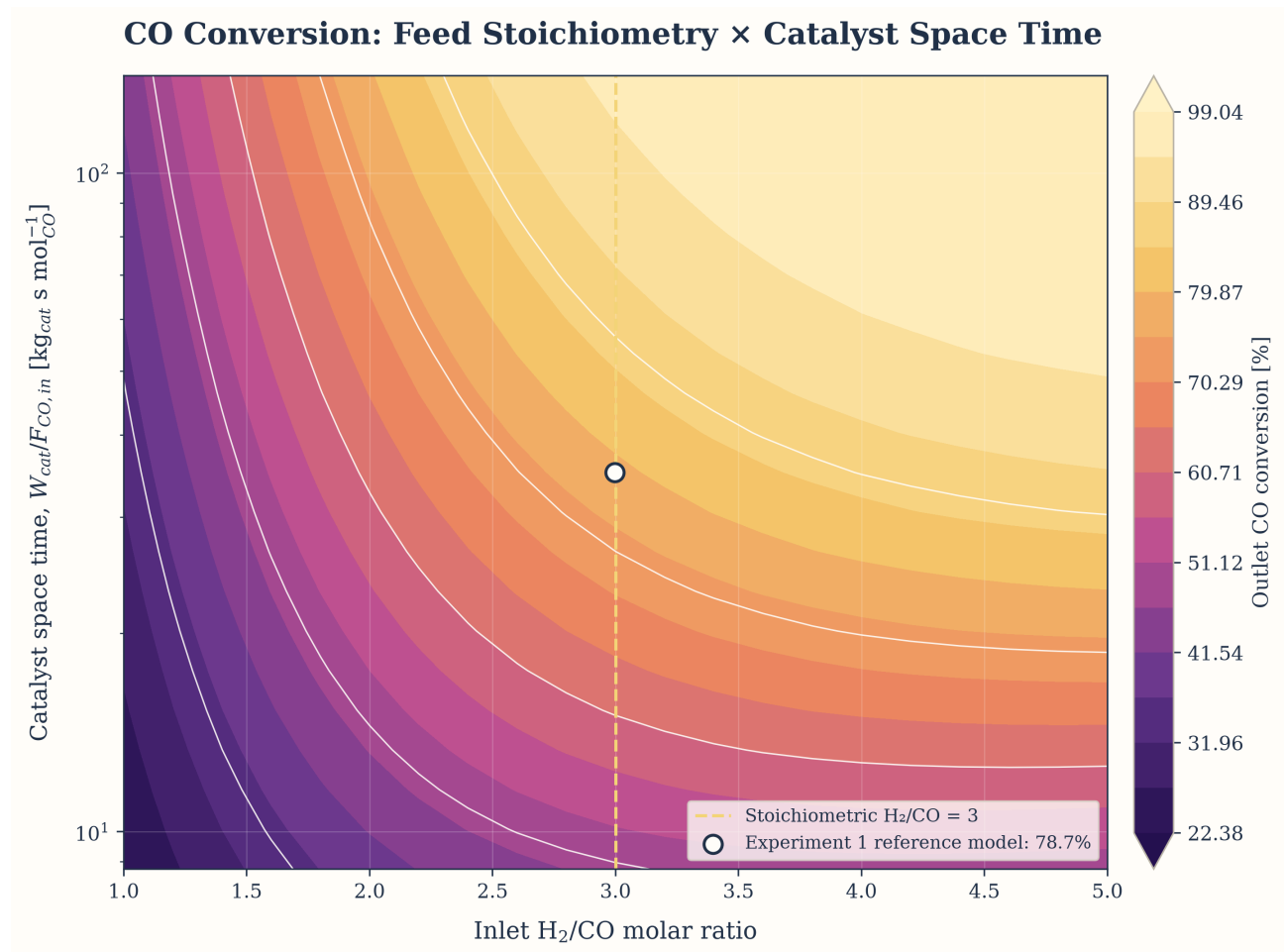
Figure 7. Full M4 predicted outlet CO conversion at 1 bar as inlet \text{H}_2/\text{CO} ratio and catalyst space time vary.
