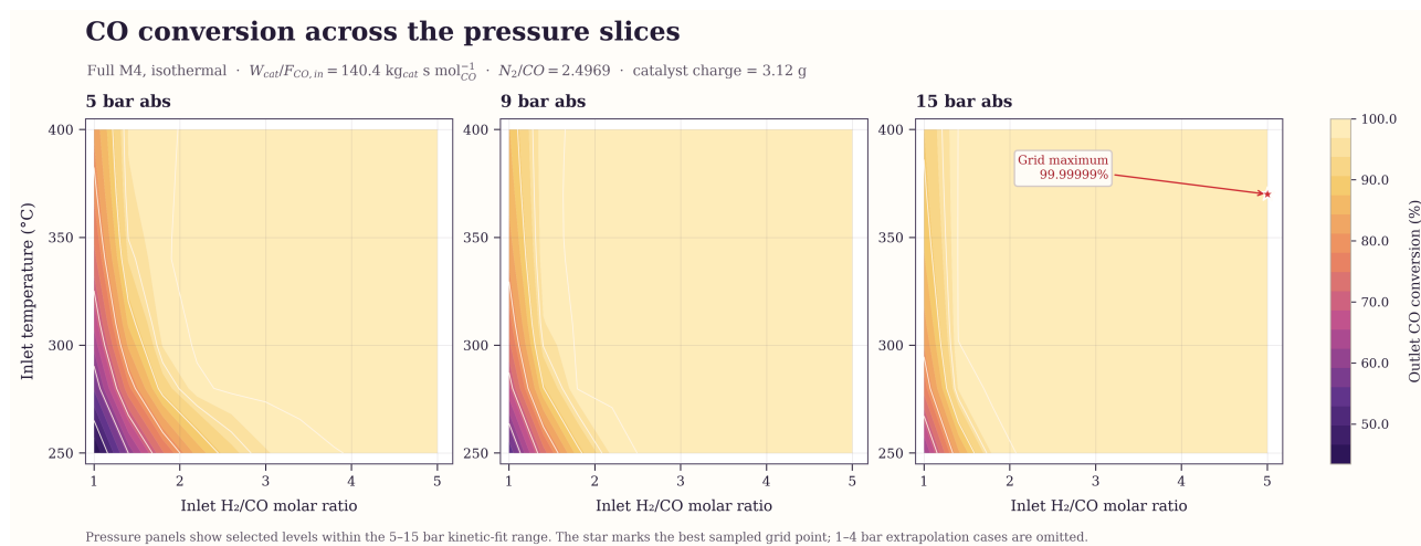
Figure 11. Pressure slices of predicted outlet CO conversion from the four-factor grid. Space time is fixed at 140.4 \text{ kg}_{\text{cat}} \text{ s mol}_{\text{CO}}^{-1} ; the star marks the best sampled point.
