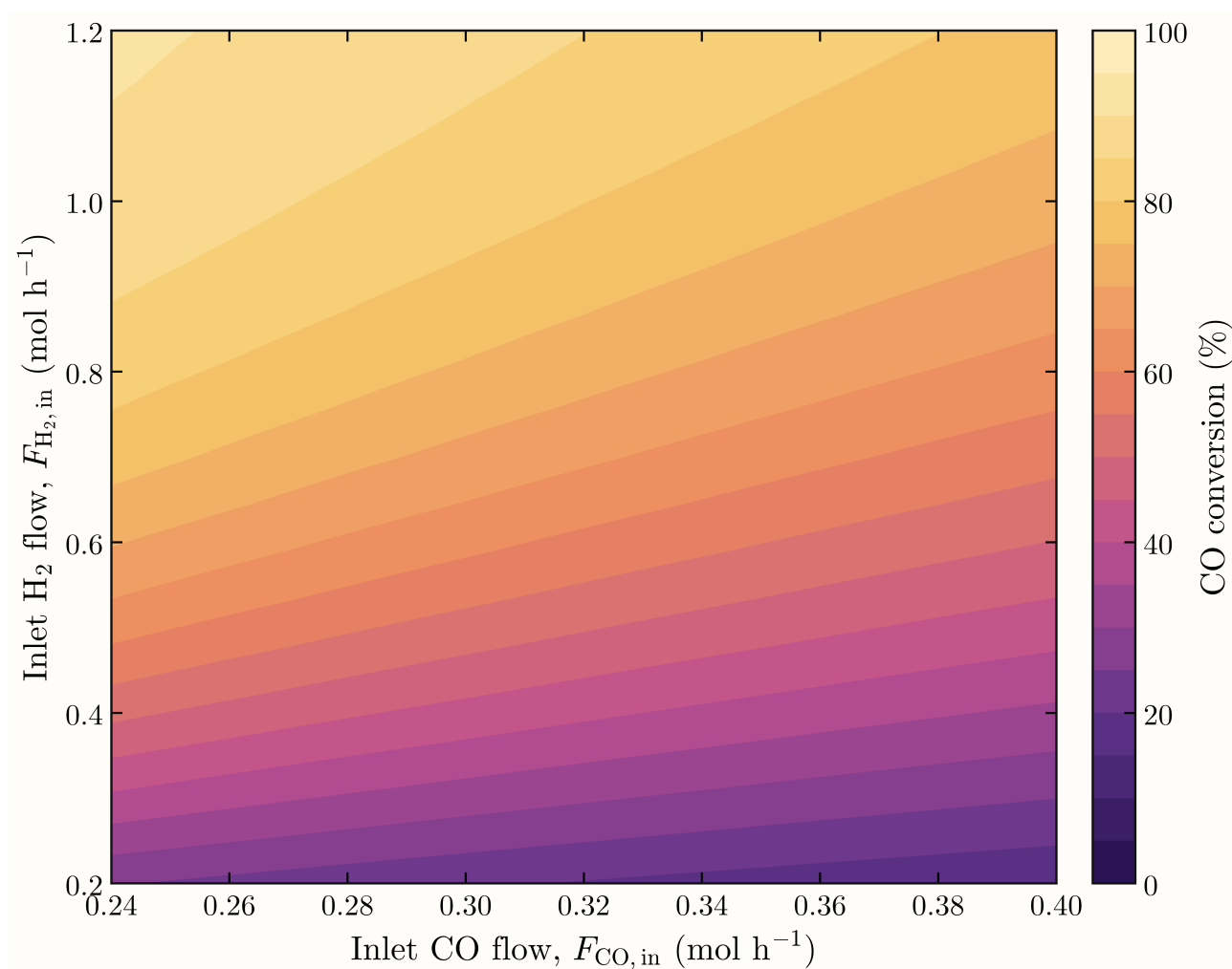
Figure 8. Full M4 predicted outlet CO conversion versus absolute inlet H 2 and CO flow; N 2 is fixed at 0.799 mol h -1 .
