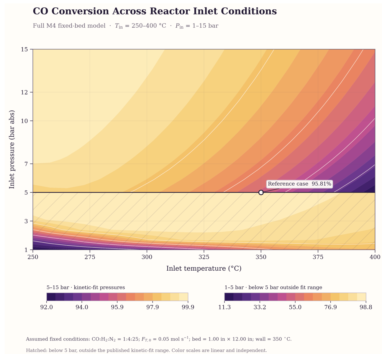
Figure 5. Full M4 sensitivity of bed-outlet CO conversion to inlet temperature and pressure.
