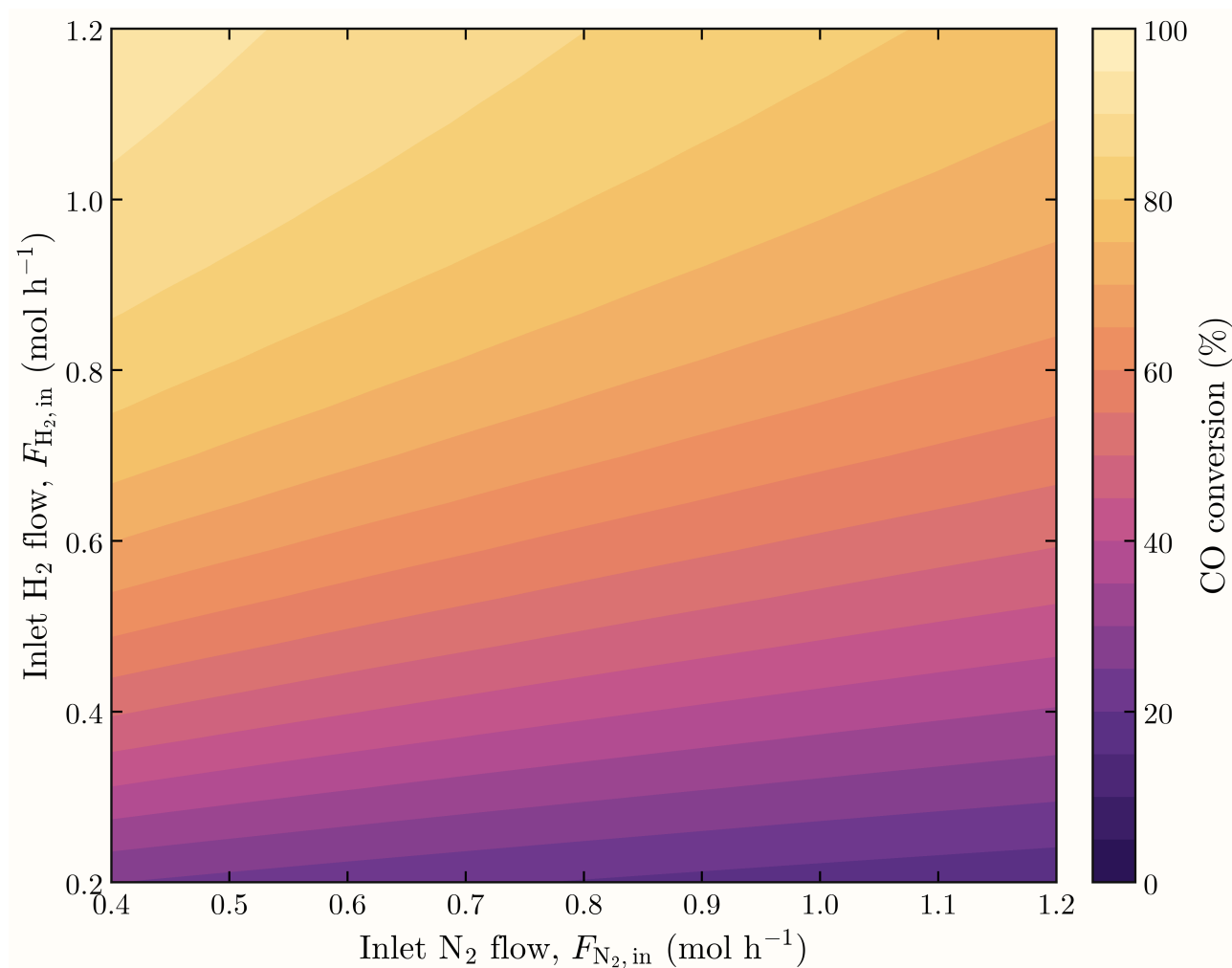
Figure 9. Full M4 predicted outlet CO conversion versus inlet H 2 and N 2 flow; CO is fixed at 0.320 mol h -1 .
