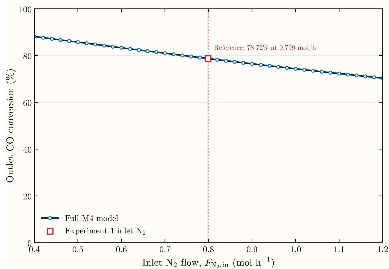
Figure 10. Full M4 predicted outlet CO conversion as inlet N 2 flow varies from 0.4 to 1.2 mol/h, with CO = 0.320 mol/h and H 2 = 0.959 mol/h fixed. The reference point at N 2 = 0.799 mol/h gives 78.72% conversion. Conditions are 350 °C, 1 bar absolute, and 3.12 g catalyst, isothermal and constant-pressure.
